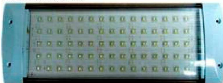
J-5300-LED Slim Roof Lamp waterproof sealed to IP66 372x138x23 mm.Recessed mount. Hole-drill:310x116 mm , Height after installed : 6mm. 75 white LEDs plus 24 blue or red LEDs. 3 lead wire Without switch.
