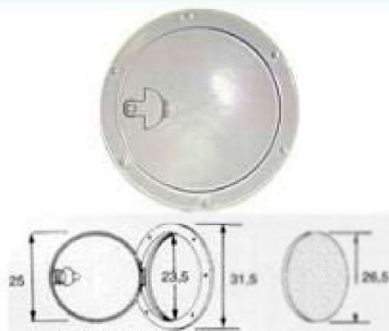
1610 : Inspection Hatch, Round
